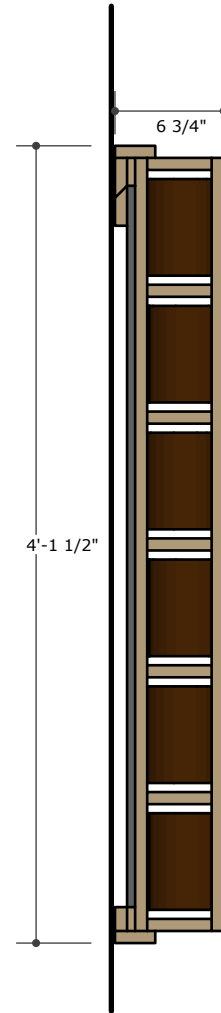
SECTION
