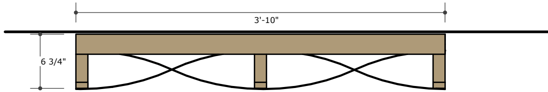
PLAN
